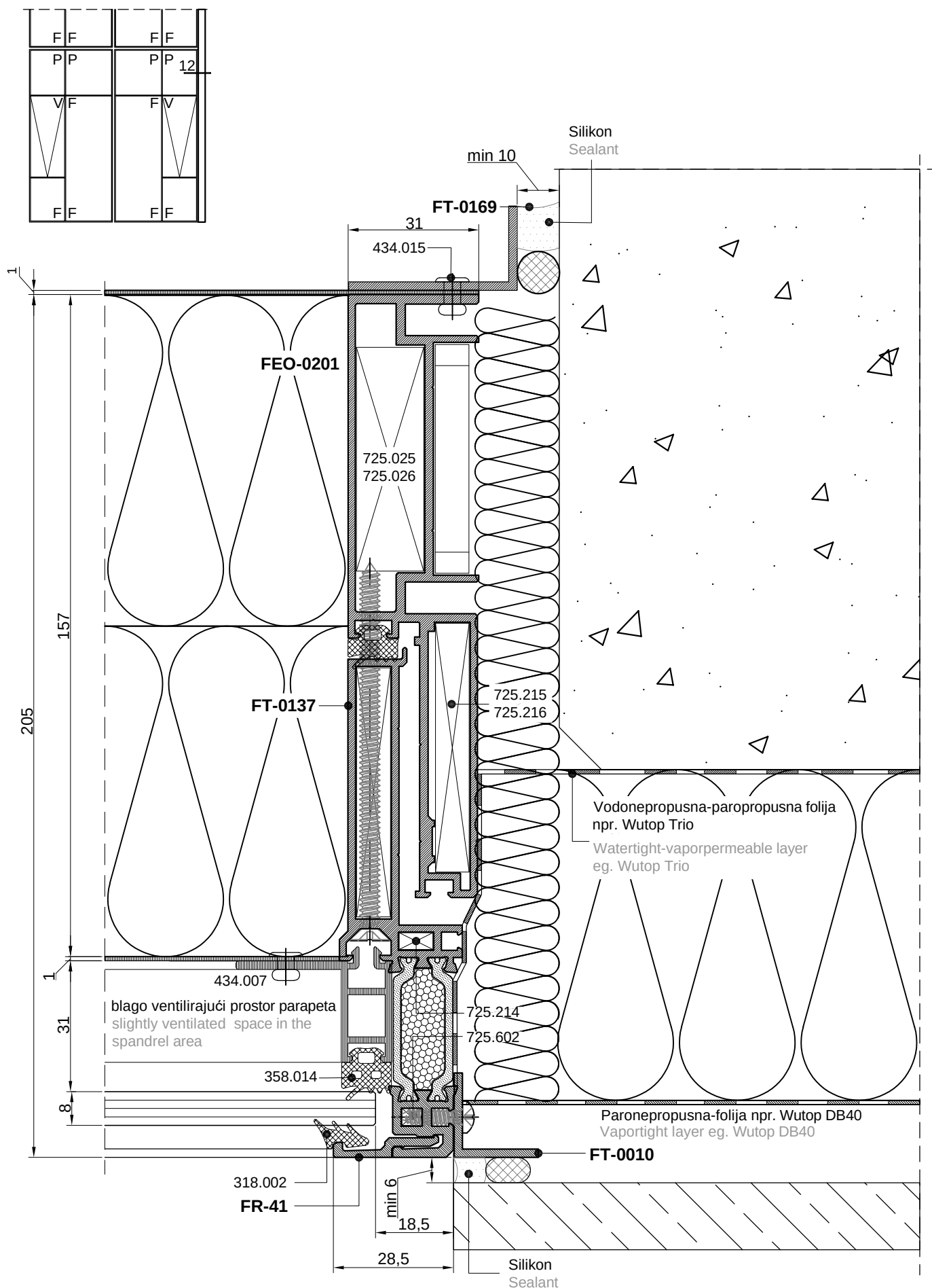
Spoj sa zidom - Presjek 12-12 Wall connection - Cross section 12-12
