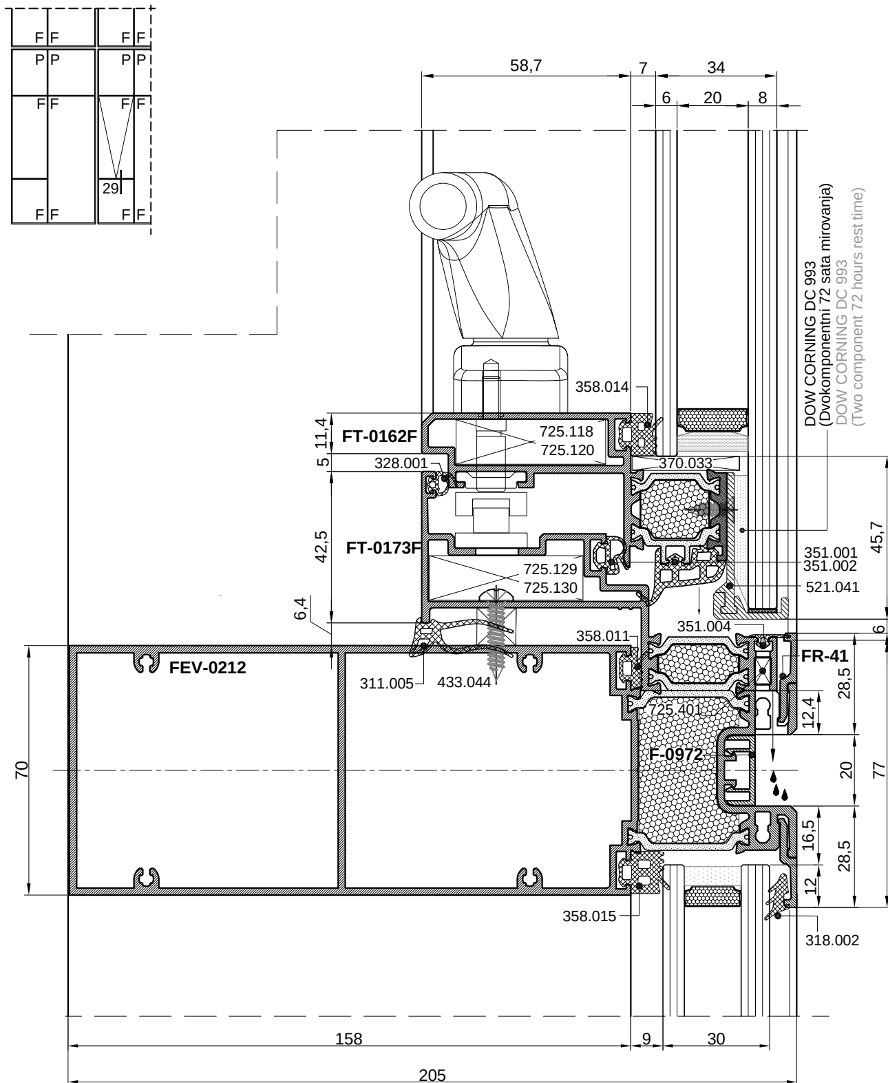
Presjek 29-29 Cross sections 29-29
