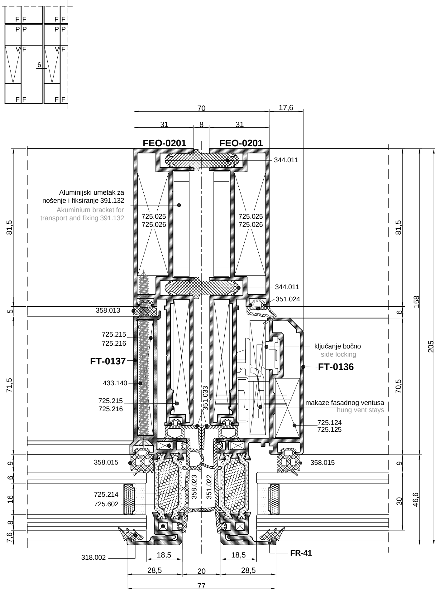
Presjek 6-6 Cross section 6-6
