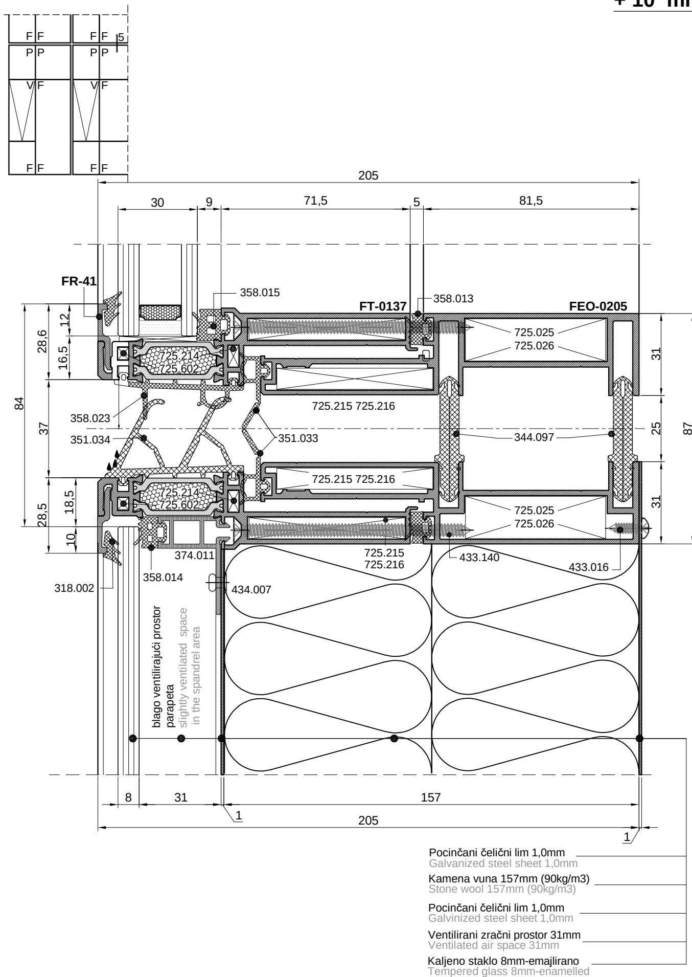
Presjek 5-5 Cross section 5-5
